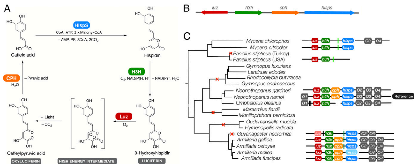
Fig. 1. Luciferin biosynthesis pathway in fungal bioluminescence and gene cluster containing key enzymes in the clade of bioluminescent fungi. (A) Proposed pathway of fungal luciferin biosynthesis and recycling. Caffeic acid is converted to hispidin by hispidin synthase (HispS) and hydroxylated by H3H, yielding 3-hydroxyhispidin (fungal luciferin). The luciferase (Luz) adds molecular oxygen, producing an endoperoxide as a high-energy intermediate with decomposition that yields oxyluciferin (caffeoylpyruvate) and light emission. Oxyluciferin can be recycled to caffeic acid by caffeoylpyruvate hydrolase (CPH). (B) Schematic depiction of the genomic cluster of N. nambi containing luciferase, H3H, hispidin synthase, and caffeoylpyruvate hydrolase ( cph ) genes. (C) Gene cluster in the clade of bioluminescent fungi. The species tree in Left is based on the comparison of protein-coding genes shared by most of the analyzed species. The red crosses mark the branches of the tree that eventually lost the ability to glow. Right shows the structure of the luciferase-containing gene cluster if such a cluster was found in the relevant genome. The genes coding for luciferase ( luz ), h3h , hispidin synthase ( hisps ), and caffeoylpyruvate hydrolase ( cph ) are colored. The lighter blue and red colors of hisps and luz genes indicate that only a partial or truncated gene was found in Armillaria mellea and Guyanagaster necrorhiza , respectively. Other genes that might belong to the cluster are named from O1 to O4 (colored in gray). Green ticks represent a cytochrome P450-like gene (different shades of green indicate different orthologous groups), and black ticks indicate other genes.
